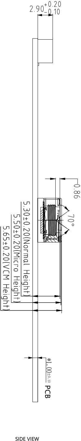
SIDE VIEW
