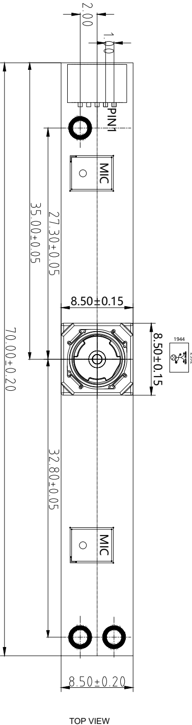
TOP VIEW
